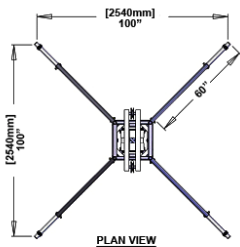
PLAN VIEW
